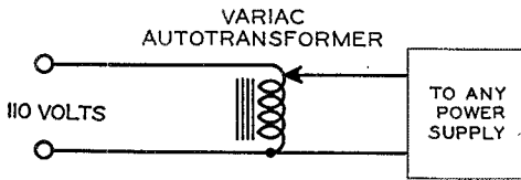
THE CIRCUIT
